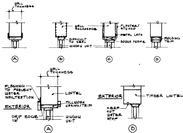
Figure 5.5: Details of window jambs (top) and heads (bottom) (Reproduced from McHenry, 'Adobe and rammed earth buildings')
