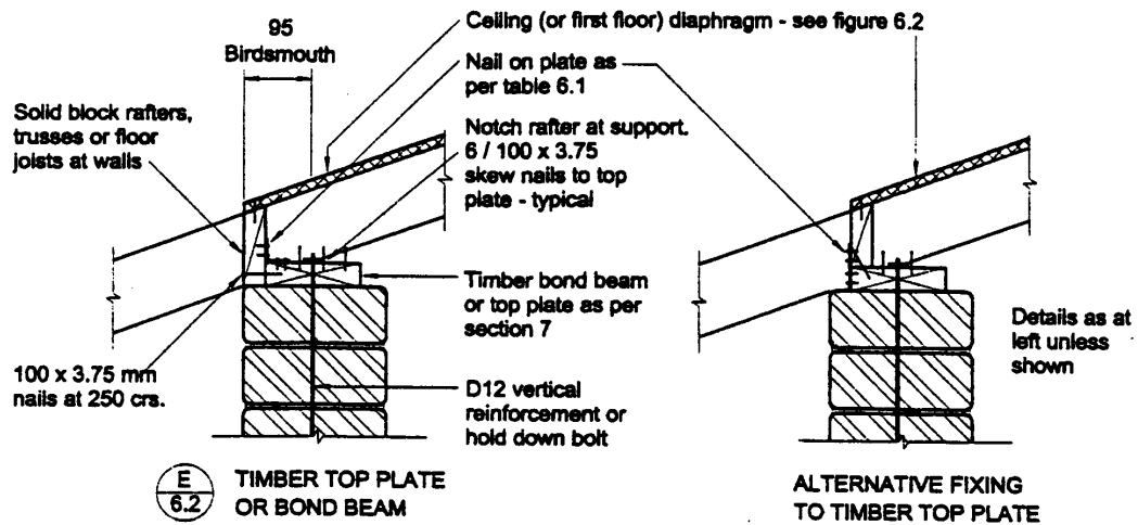
Figure 5.9: Timber bond beam-roof connection (Reproduced from NZS 4299, 'Earth buildings not requiring specific design')
